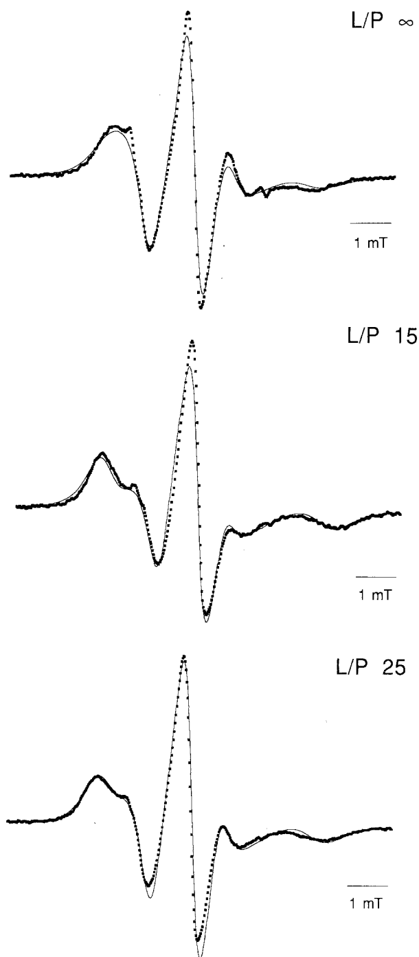
Fig. 2. ESR spectra of 12-SASL in DOPC bilayers at 10°C with various L/P ratios (mole/mole) of M13 coat protein. The dotted lines are the experimental data and the straight lines represent the simulations. For the simulations the components for the hyperfine coupling tensor and g tensor were used as described in Material and methods. The values for D_{\perp} are 3.4 \times 10^{-7} \text{ s}^{-1} for L/P \infty , 2.4 \times 10^{-7} \text{ s}^{-1} for L/P 25 and 1.9 \times 10^{-7} \text{ s}^{-1} for L/P 15. The order parameter was taken to be zero in all spectra
